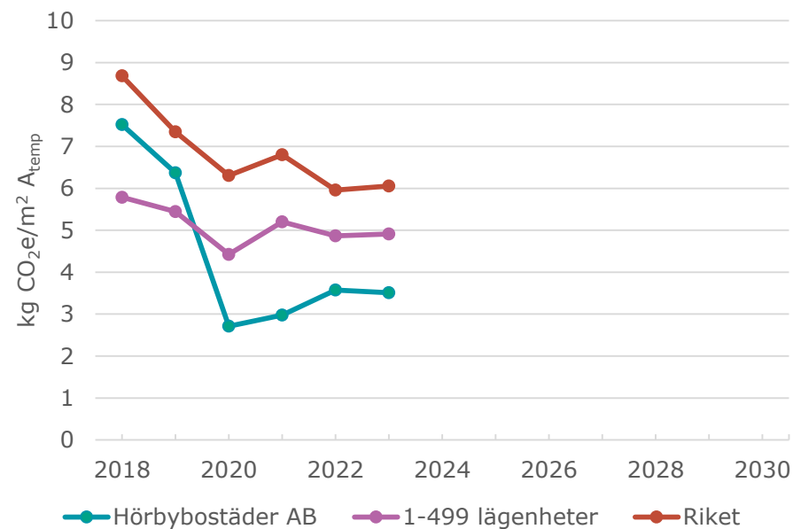
Diagram 4.5.2 Koldioxidprestanda Location Based
