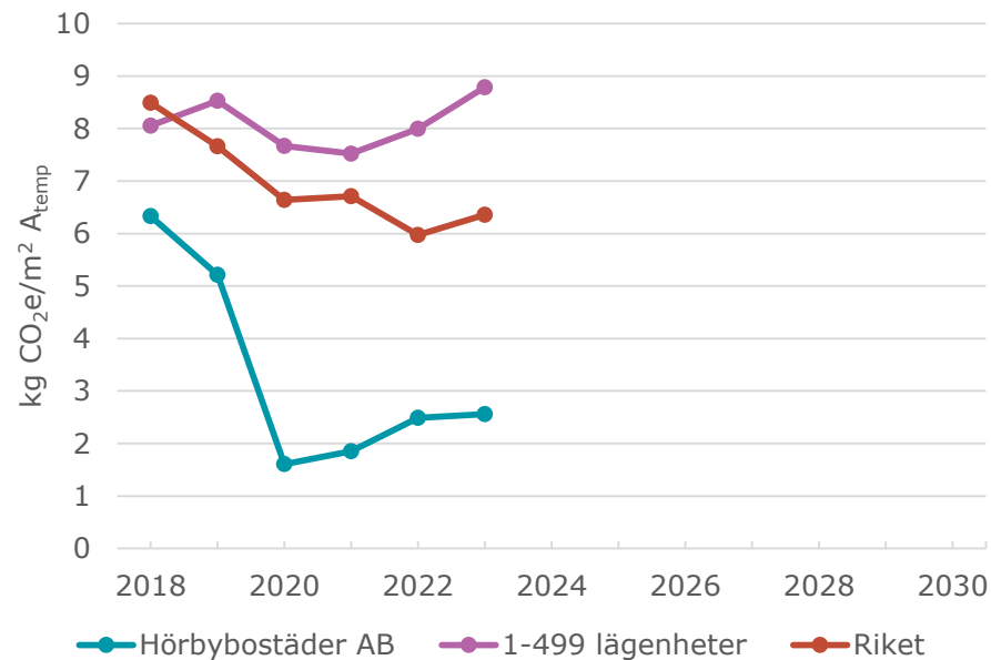
Diagram 4.6.2 Koldioxidprestanda Market Based
